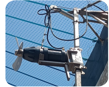
Agitators/ Mixers
